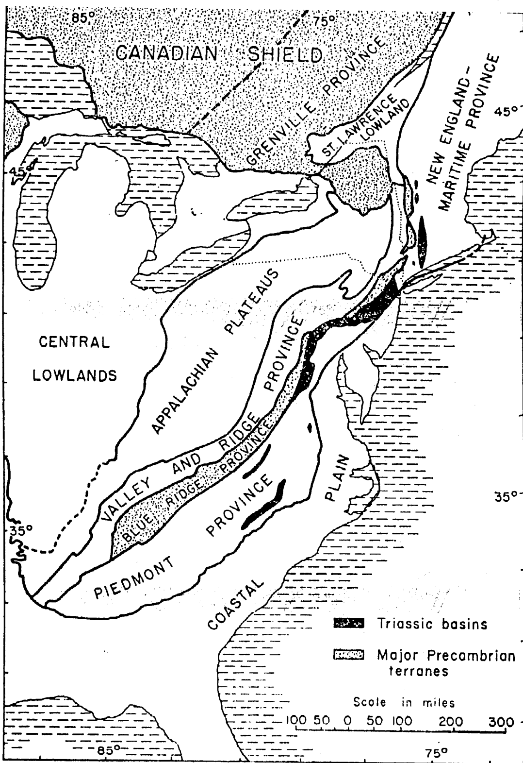
FIGURE 2. Physiographic and tectonic provinces of part of eastern North America
